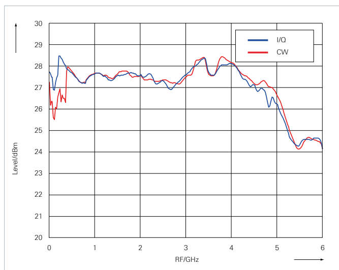
Measured maximum output power vs. frequency
